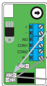
JUMPER J2
