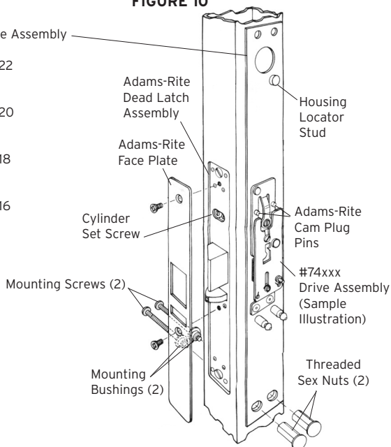
Combination Lock Side
