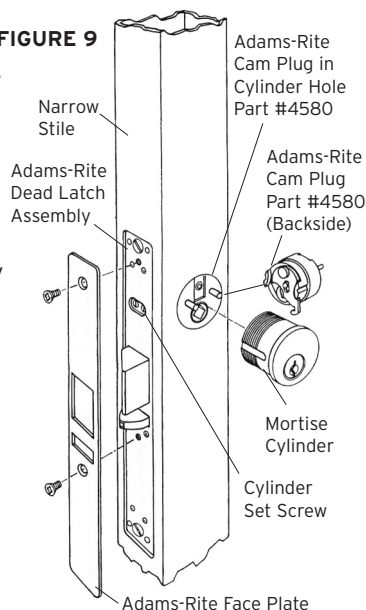
Combination Lock Side
