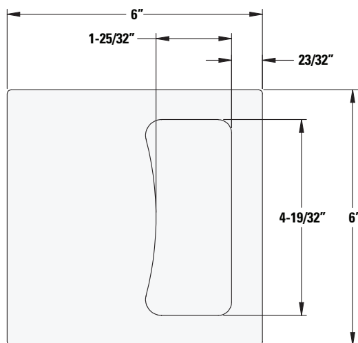
FRONT VIEW 1111C
