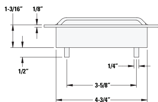
TOP VIEW 1111C
