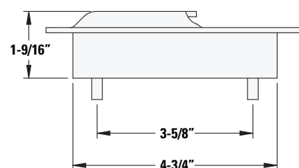
SIDE VIEW 1111C
