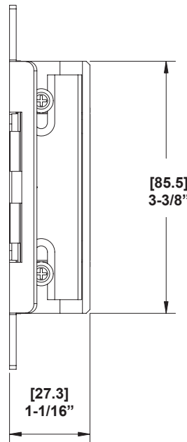
Side View
