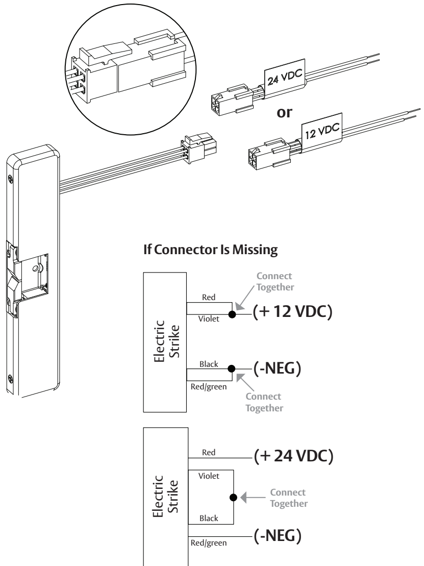
Diagram 2: 12V to 24V Conversion
